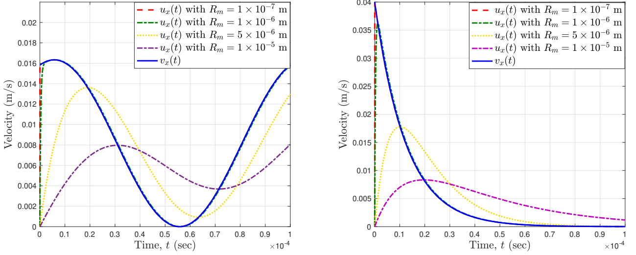
Figure 4. Comparison between instantaneous velocities u_x(t) (accounting for mass and viscosity) for different molecule radii and the desired velocity v_x(t) . The sinusoidal and optimized fields from Fig. 2(a) and Fig. 3(b), respectively, are assumed.
